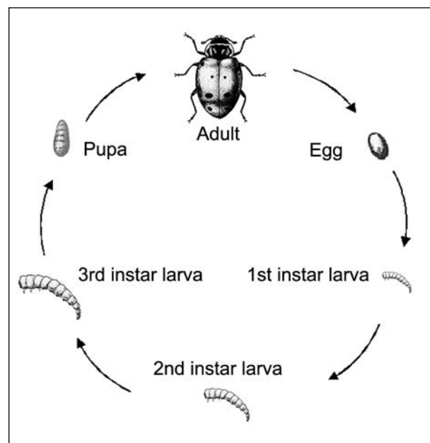
Figure 10. Complete metamorphosis.
